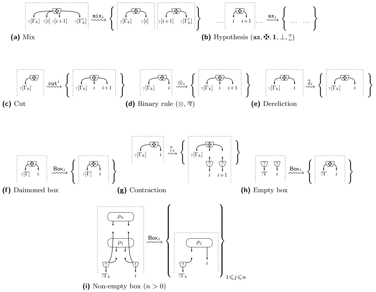
■ Figure 11 Actions of elementary paths on \mathbf{X} -cells and on a box in \text{qDiLL}_0^{\mathbf{X}} .
