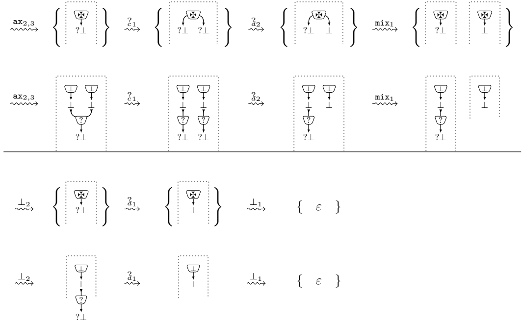
■ Figure 9 The path \text{Box}_2 \ ?_{d_1} \ \text{Box}_2 \ \text{?}_{d_2} \ \text{mix}_1 \ \text{ax}_{2,3} \ ?_{c_1} \ ?_{d_2} \ \text{mix}_1 \ \perp_2 \ ?_{d_1} \ \perp_1 witnessing that \rho \in \mathcal{T}(R) (continued from Figure 8).
