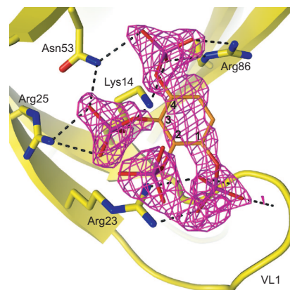
Figure 2. Binding of Bz(1,2,3,4)P 4 to the PKB \alpha PH domain in the crystal structure. Unambiguous |F_o| - |F_c| electron density (magenta), contoured at 2.25\sigma , is observed, covering all atoms of the ligand. Protein and ligand atoms are colored with purple phosphorus atoms, red oxygen atoms, and blue nitrogen atoms. Hydrogen bonds are indicated as black dotted lines.
