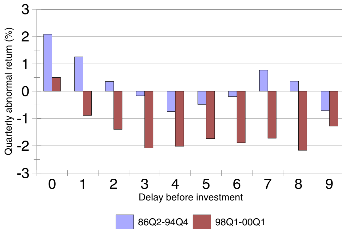
Figure 2. Abnormal returns after consecutive non-negative surprises
