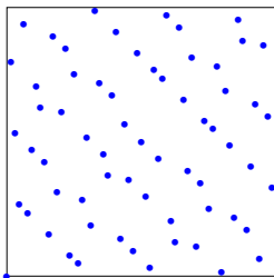
64 Sobol' points
