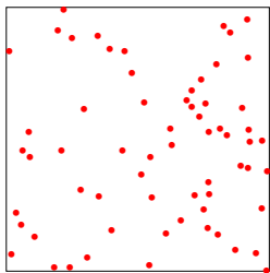
64 random points
