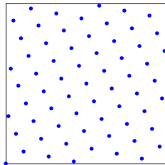
64 lattice points
