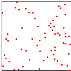
64 random points
