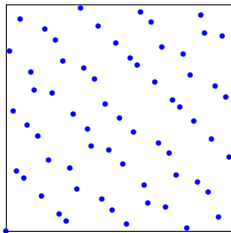
64 Sobol' points
