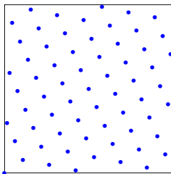
64 lattice points
