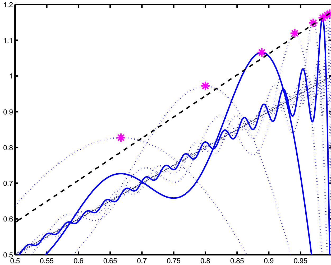
Gibbs' phenomenon (up to 256 terms)
