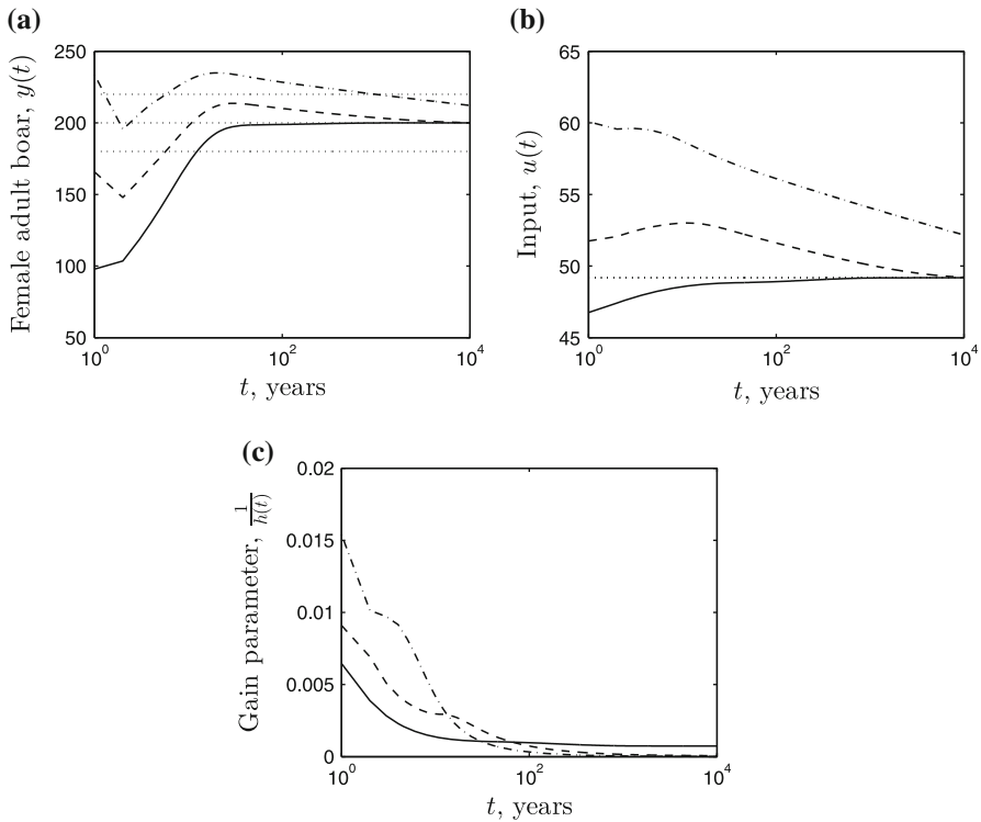
Fig. 11 Adaptive integral control (3.26) applied to the wild boar matrix PPM of Example 1 with different initial triples (x^0, w^0, h^0) . See Example 6. In each plot the solid , dashed and dashed–dotted lines are corresponding simulations. a Observations. The dotted lines are the reference r = 200 and r \pm 10\% . b Filtered input signals and limiting input r/G(1) in dotted line. c Adaptive gain parameters g(t) = \frac{1}{h(t)}
