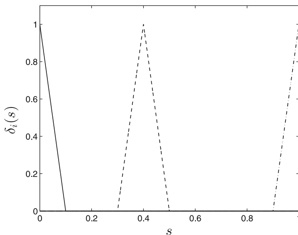
Fig. 15 Three sample hat functions defined by (5.26) with \alpha = 0 , \beta = 1 and N = 10 . The functions \delta_1 , \delta_5 and \delta_{11} are plotted in solid , dashed and dashed-dotted lines respectively
