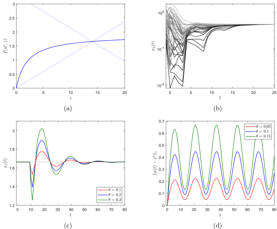
Figure 5.1: Numerical simulations illustrating Example 5.1. (a) Graph of the nonlinearity z \mapsto f(u^e, z) in (5.3). The straight lines have slope \pm p and intersect the graph of f at z = z^e . (b) Plots of x_4(t) against t for varying [[x(0), x(-1)] \in \Gamma , with logarithmic scale on the vertical axis. The dotted line is x_4^e . (c) Plots of x_1(t) against t for varying \theta . (d) Plots of \|x(t) - x^e\|_1 against t for varying \theta .
