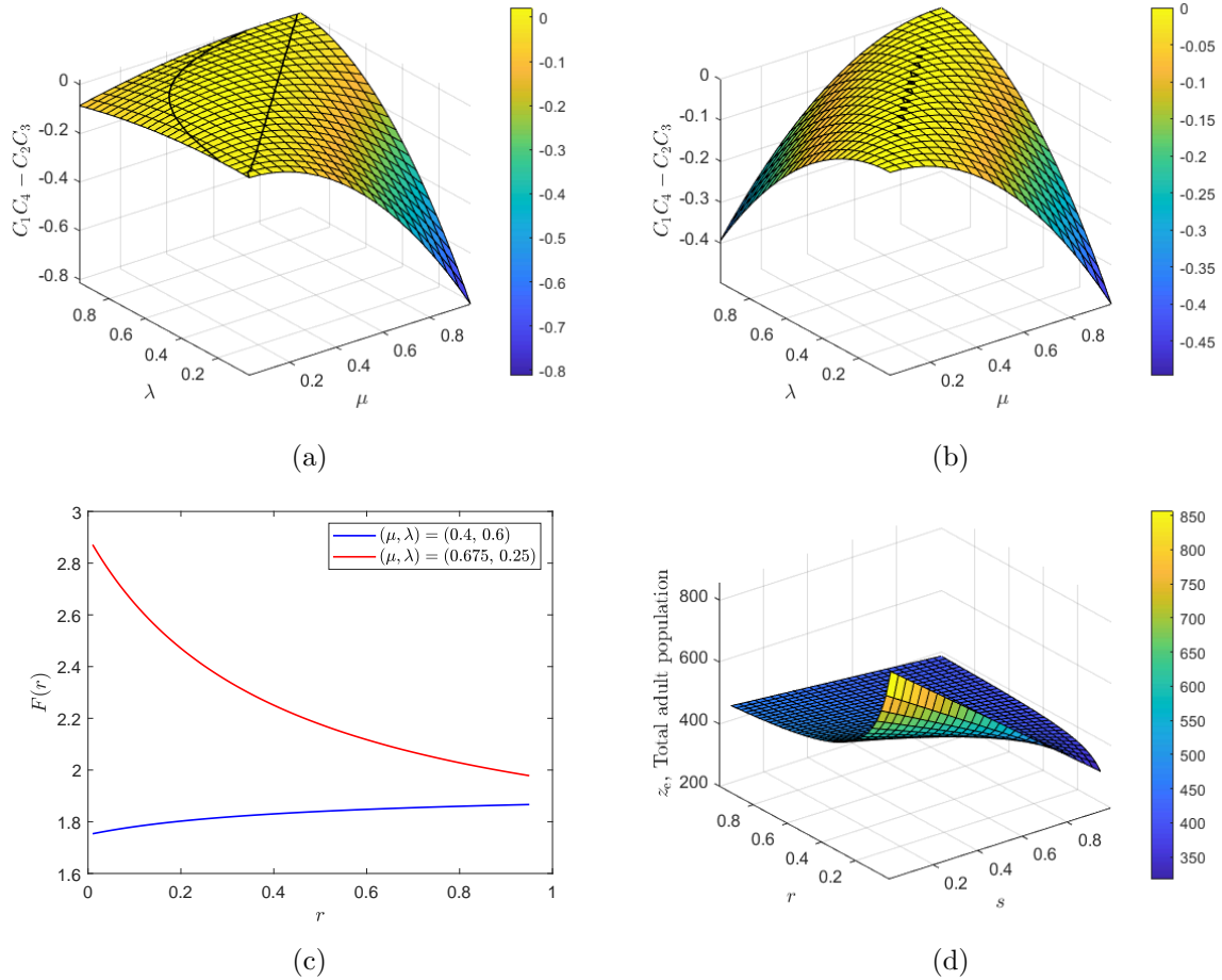
Figure 5.2: Numerical simulations illustrating Example 5.2. (a) and (b) Surface plots of C_1C_4 - C_2C_3 in (5.6) against varying \lambda and \mu for s = 0.9 and s = 0.55 . (c) Graphs of F(r) against r for different (\mu, \lambda) pairs, with fixed s = 0.9 . (d) Surface plot of asymptotic adult population size z^e against varying r and s , here \lambda = 0.9 , \mu = 0.7 , and f(z) = \frac{1.1z}{1+0.01z} .
