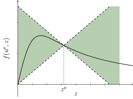
Figure 4.1: Illustration of the sector condition (4.1). The dashed lines have slope \pm p .
