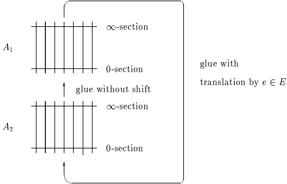
FIGURE 1. Glueing of the surface \bar{A}_u
