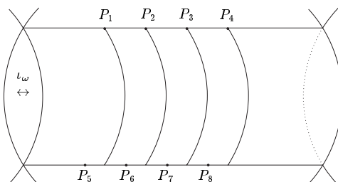
FIGURE 2. The involution \iota_\omega
