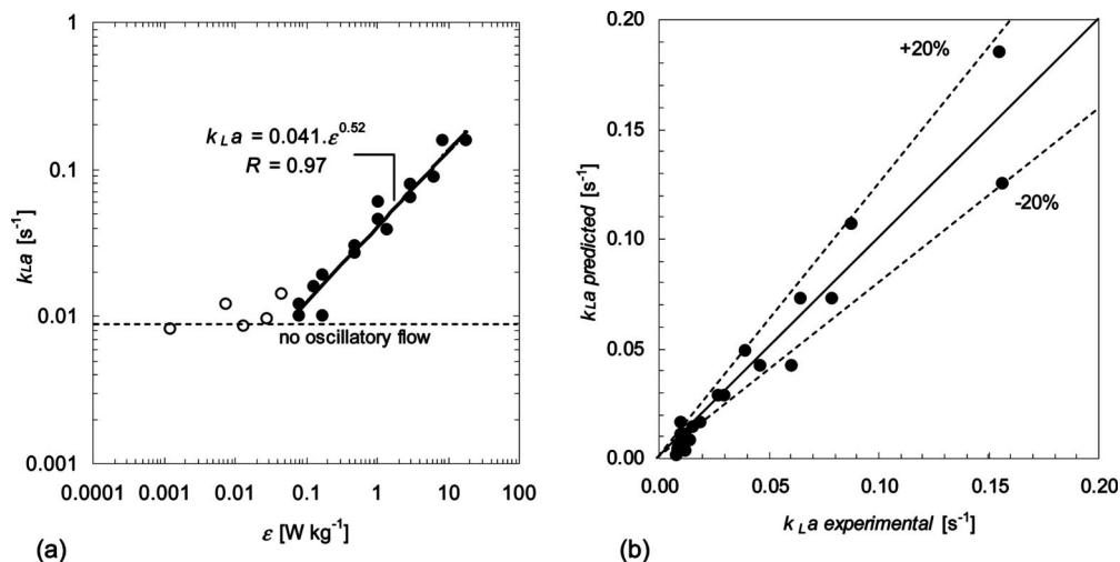
Figure 11. Correlation of k_La with the cycle-average “turbulent” kinetic energy dissipation ( \bar{\epsilon} ) in the OMT. (a) Log–log plot of k_La versus \bar{\epsilon} ; the dots with white background represent values not considered in the correlation and obtained at Re_o < 200 . (b) Parity plot comparing the predicted k_La values with the experimental k_La using eq 10, line of parity (—), and (---) represents 20% either side of parity.
