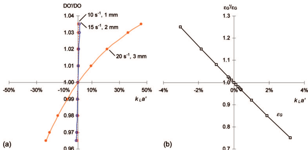
Figure 9. Sensibility analysis of k_La values for variations in the dissolved oxygen concentration (DO) and gas holdup ( \varepsilon_G ) in the range given by the maximum standard deviation obtained between experimental duplicates.
