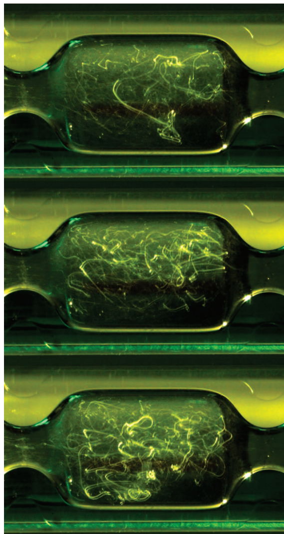
Figure 4. Pathlines defined by bubbles moving in a horizontal OMT for one complete oscillation cycle ( f = 15 \text{ s}^{-1} , x_0 = 2 \text{ mm} ).
