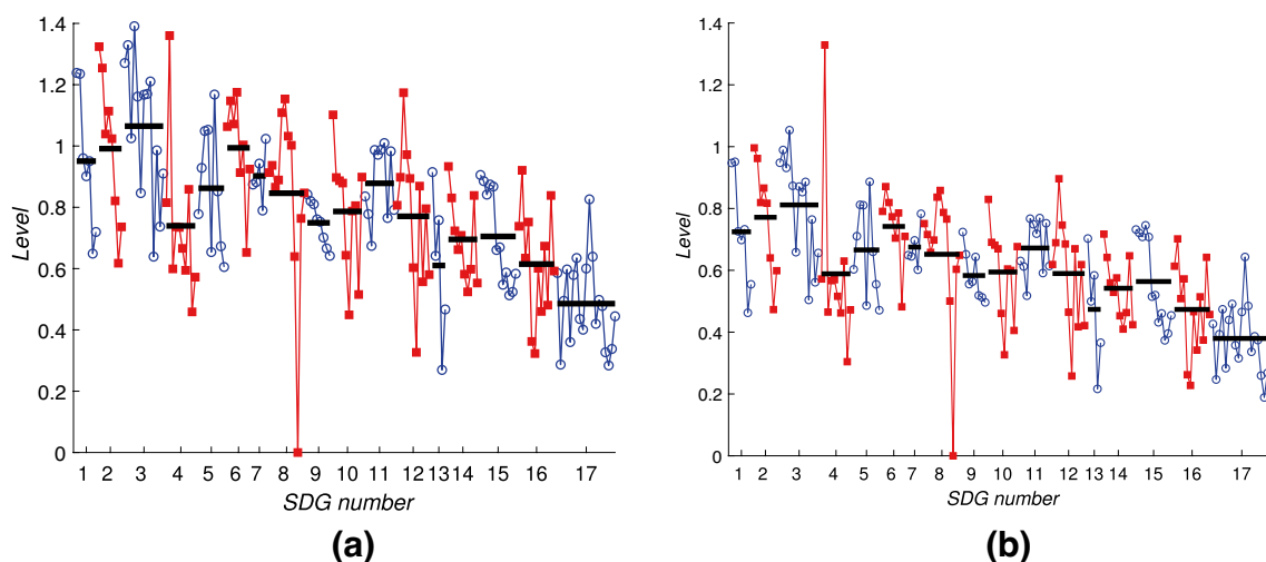
Fig. 13 Levels h_i for each target i = 1, \dots, 169 , together with averages for each SDG (black horizontal lines) computed for \alpha = 1 . a Bangladesh matrix \tilde{A}_{\text{BGD}} ; b Indonesia matrix \tilde{A}_{\text{IDN}} . Each matrix is
