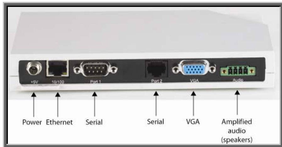
Figure 2-ConnectPort Back Panel
