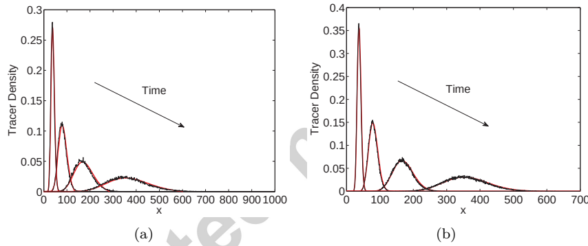
Figure 3: A comparison of the expected occupancy of tracer particles on an exponentially growing domain in the stochastic and deterministic regimes at different times. The red curves represent the solution of the Fokker-Planck equation (23) and the (noisy) black curve represents the expected density of tracer particles averaged over 10,000 realisations of the individual based model. In both cases L(0) = 30 , with tracer particles initially between 15 \leq x \leq 20 . The rate of element proliferation is b = 0.05 and the curves are plotted at t = 15, 30, 45, 60 . (a) \Delta = 1 , (b) \Delta = 1/2 .
