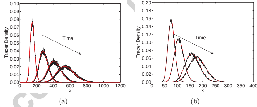
Figure 11: A comparison of the expected occupancy of tracer particles on domains growing according to (a) linear and (b) Gompertzian growth in the stochastic and deterministic regimes at different times. The coefficients of the FPE solved to find the red curves are determined using the coefficient estimation approach and are those displayed in Fig. 10. Figure descriptions and initial conditions are as in Fig. 3. Parameters are as in Fig. 10. \Delta = 1/2 in both cases.
