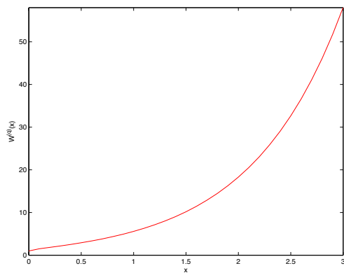
(a) X is \alpha -stable process with \alpha = 0.5
