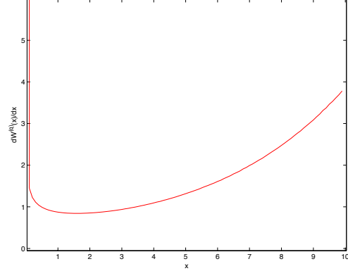
(b) X is \alpha -stable process with \alpha = 1.75
