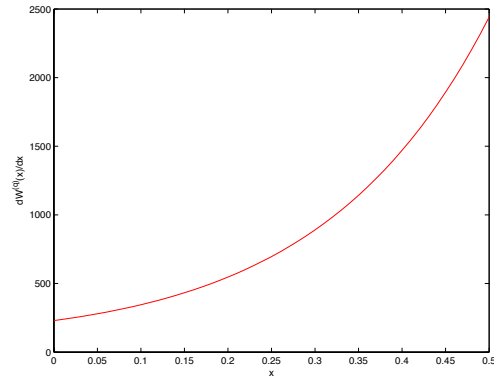
(b) X is compound Poisson process with drift d = 0.05 .
