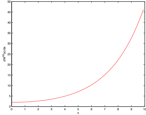
(a) X is standard Brownian motion.
