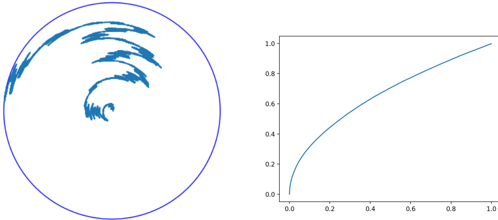
FIGURE 1. A simulation of a solution of the SDE (2.1) (left) and its radius (right), up to the first exit time of a ball. These simulations already appeared in the paper [1] by the same authors.
