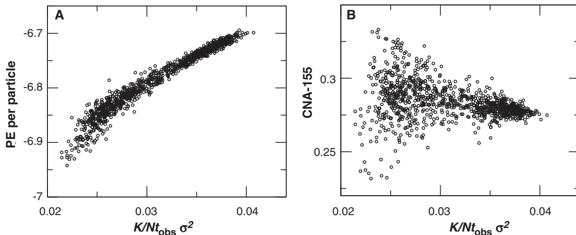
Fig. 5. Test of correlation between space-time order parameter and potential energy and icosahedral order. (A) Potential energy per particle in units of \varepsilon versus dynamical order parameter K of a trajectory. (B) Icosahedral order, as quantified by the CNA-155 parameter of the common neighbor analysis, as a function of K . Results are for trajectories at k_B T/\varepsilon = 0.6 , t_{\text{obs}} = 40\tau , and N = 150 .
