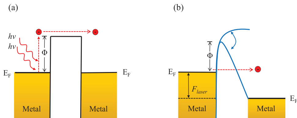
Figure 2. Mechanisms of optical-field-driven tunneling. a) Multiphoton emission. An electron absorbs the energy of a number of photons to overcome the barrier for photoemission. E_F , Fermi level; \Phi , barrier height. b) Optical-field tunneling emission. A strong optical field induces a periodically oscillating barrier at an optical-frequency of \omega . When the optical field is strong enough to create a penetrable tunneling barrier, electrons tunnel from the Fermi level in a fraction of a negative half optical-cycle.
