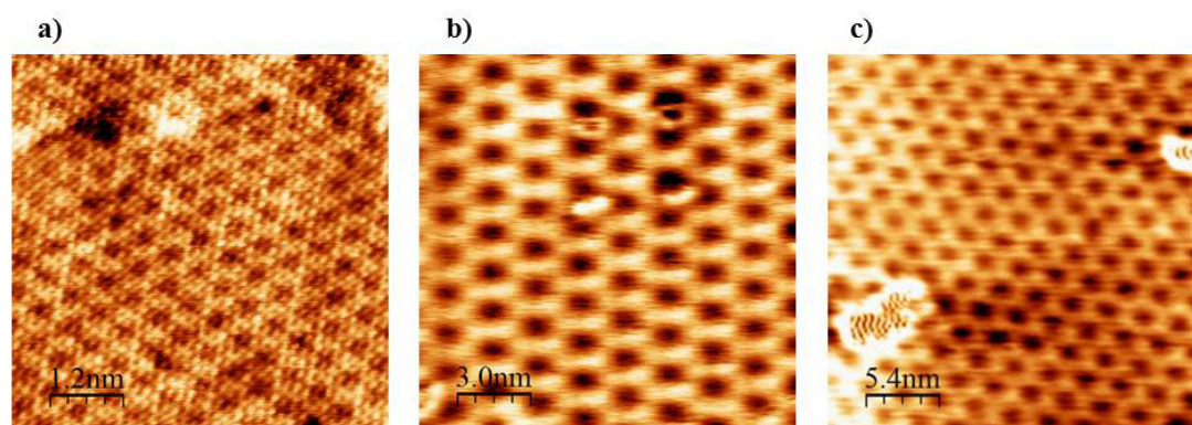
Figure V.28. STM images of SLG grown from C 60 on: (a) Pt(111), (6 × 6) nm, 0.11 V, 2.3 nA. (b) Ir(111), (15 × 15) nm, 1.2 V, 2.6 pA and (c) Cu(111), (27 × 27) nm, −0.4 V, 2.7 pA. In every image different moiré superstructures are shown.
