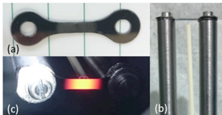
Figure V.21. A glassy carbon filament (a) is mounted on an UHV electrical feedthrough (b) and resistively heated (c). T is simultaneously measured with an optical pyrometer and a type-C thermocouple located on the back side.
