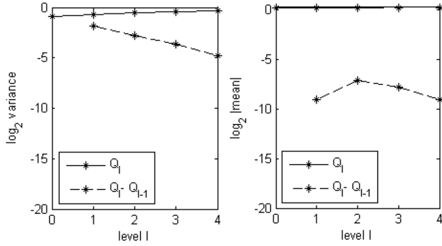
Figure 6: Plots of \mathbb{V}[Q_\ell] and \mathbb{V}[Y_\ell] (left plot), as well as \mathbb{E}[Q_\ell] and \mathbb{E}[Y_\ell] (right plot) in the case \lambda = 0.3 , \sigma^2 = 1 , m_{\text{KL}} = 1400 in 2D, with m_0 = 4 and Q = -k \frac{\partial p}{\partial x_1} at the centre of the domain.
