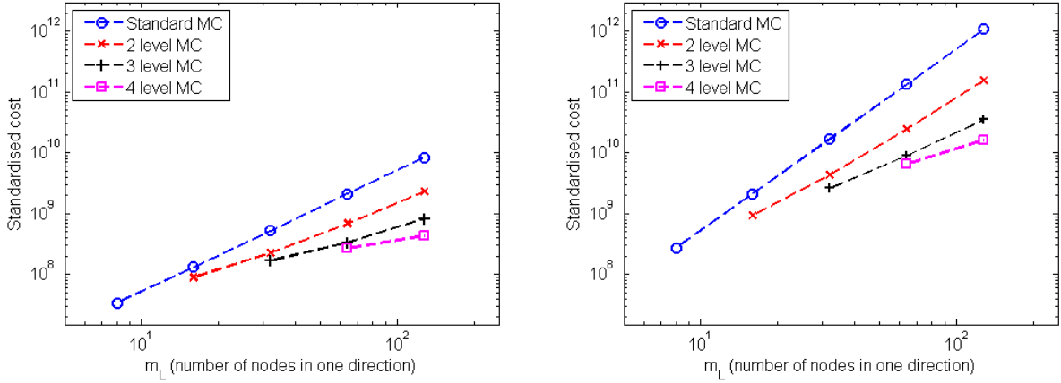
Figure 4: Plots of the standardised cost (scaled by 1/C^* ) versus m_L for a fixed tolerance of \delta = 10^{-3} for the maximum standard deviation of the MLMC estimator for \mathbb{E}[k_{\text{eff}}] for \lambda = 0.3 , \sigma^2 = 1 , m_{\text{KL}} = 1400 assuming \gamma = 1 (left plot) and \gamma = 1.5 (right plot).
