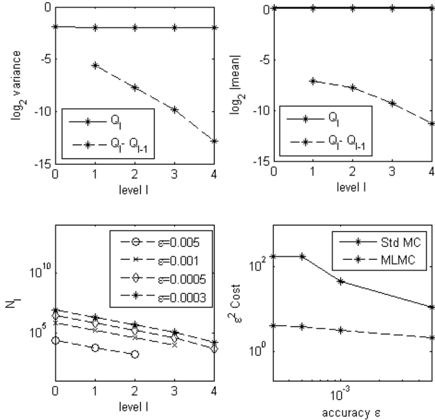
Figure 3: Performance plots for \lambda = 0.3 , \sigma^2 = 1 , m_{\text{KL}} = 1400 and m_0 = 8 in 2D. The quantity of interest is the effective hydraulic conductivity k_{\text{eff}} defined in (4.1).
