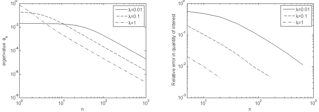
Figure 1: Left: Plot of the KL eigenvalues in decreasing order as a function of their index, for different choices of the correlation length \lambda and for d = 1 . Right: Corresponding relative error (or bias) |\mathbb{E}[k_{\text{eff}}(Z)] - \mathbb{E}[k_{\text{eff}}(Z_{m_{\text{KL}}})]|/\mathbb{E}[k_{\text{eff}}(Z)] in a typical quantity of interest (here the effective hydraulic conductivity k_{\text{eff}} defined in Section 4) as a function of the number of KL modes included.
