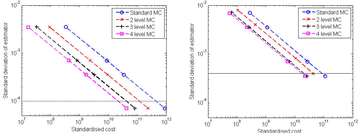
Figure 5: Same test case as in Figure 4. Standard deviation of the MLMC estimator \widehat{Q}_L^{ML} versus the standardised computational cost for fixed m_L = 128 . The horizontal line represents the estimated spatial discretisation error on this grid. Quantities of interest: \mathbb{E}[k_{\text{eff}}] (left plot) and \mathbb{E}\left[-k \frac{\partial p}{\partial x_1}\right] at the centre of the domain (right plot).
