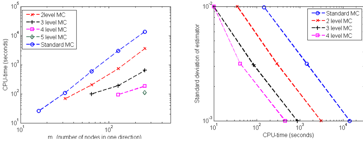
Figure 7: Same plots as in Figures 4 and 5 for \lambda = 0.1 , \sigma^2 = 1 , m_{\text{KL}} = 500 , but using actual CPU time in seconds to quantify the cost (Matlab implementation running on a 3GHz Intel Core 2 Duo E8400 processor with 3.2GByte of RAM). Left plot: \mathbb{E}[k_{\text{eff}}] , with fixed maximum standard deviation 10^{-3} . Right plot: \mathbb{E}[k_{\text{eff}}^2] , with m_L = 256 .
