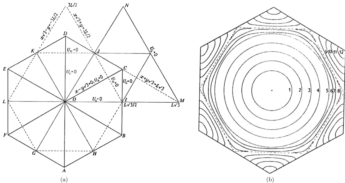
Figure 3. Hexagonal planforms for thermal convection as described in Chandrasekhar's book (Chandrasekhar, 1961/1981). Copyright © Oxford University Press. (a) Detailed construction of a hexagonal planform (page 49). (b) Contours of vertical fluid velocity within a single convection cell (page 50). This follows the earlier work by Christopherson (1940) and Pellew and Southwell (1940).
