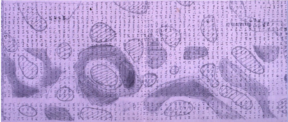
Figure 1. Detail of page AMT/K/3/8 showing a contour plot constructed and shaded by hand from the numerical solution of a model for morphogenesis. Although the pattern is a disordered snapshot and probably has not settled to equilibrium, a roughly hexagonal pattern of small hatched regions can be identified slightly to the left of the centre of the image. Copyright © W.R. Owens.
