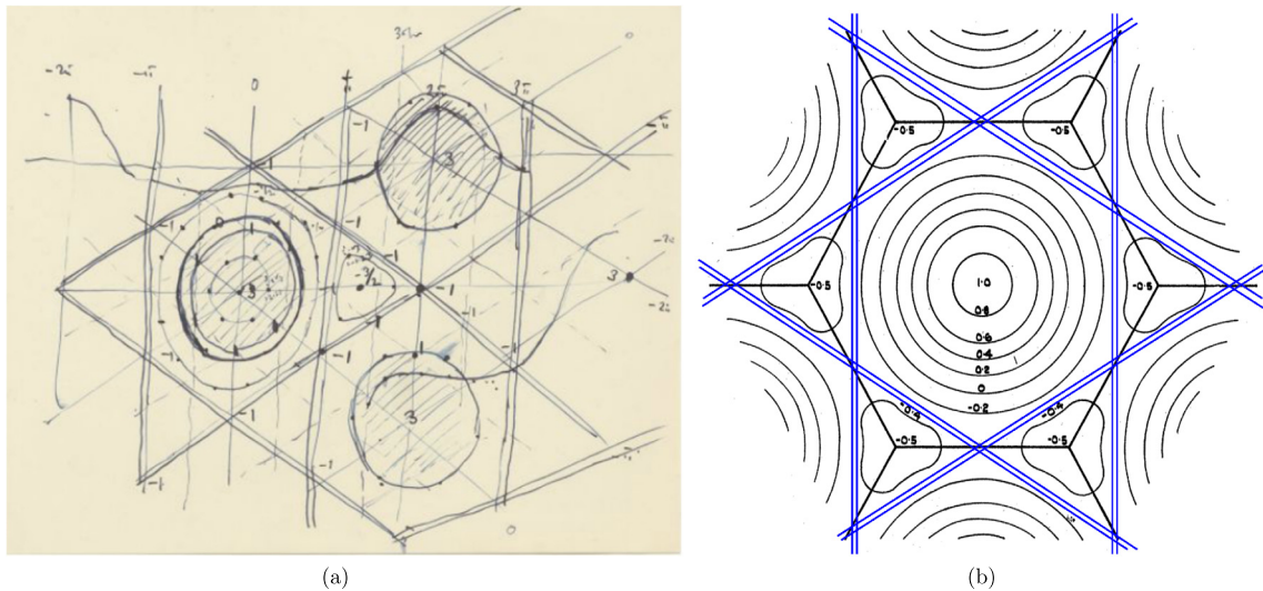
Figure 2. Two sketches of hexagonal planforms for patterns. (a) Sketch by Turing, taken from AMT/C/27/19a. Copyright © W.R. Owens. (b) Figure 3 from Pellew and Southwell (1940) following Christopherson. The pairs of blue thick solid lines are added to (b) show the relation between the figure as plotted by Pellew and Southwell and the sketch in (a) by Turing.
