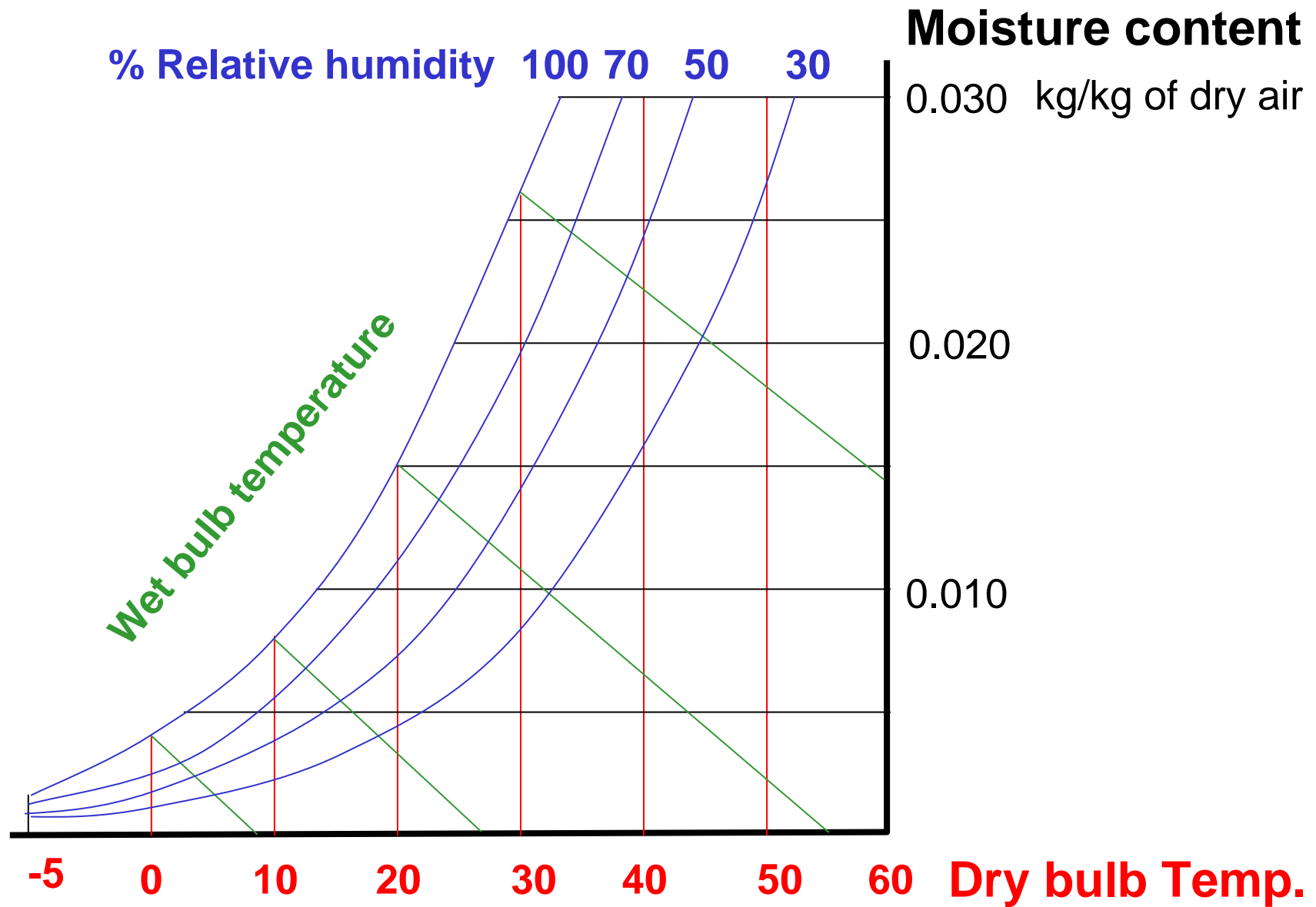
Psychrometric chart
